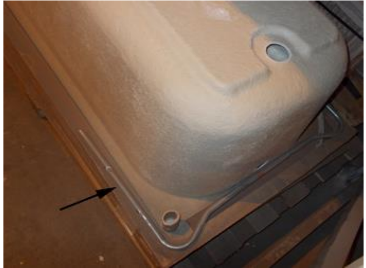
Legs screwed to rim of bath Fixings pack stapled to underside
